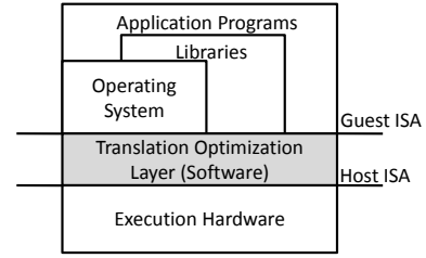
Fig. 1. HW/SW interface in co-designed processors
