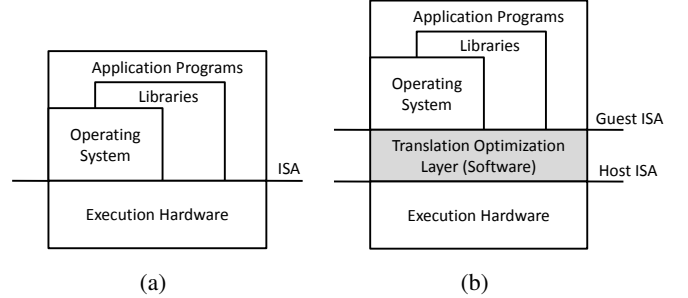
Fig. 1: HW/SW interface in processors: a) Conventional; b) Co-designed.
